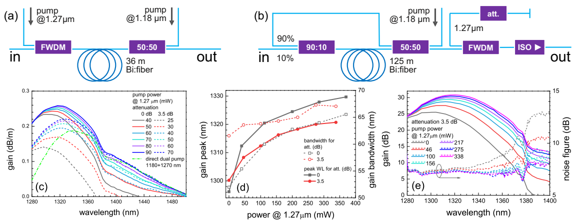
Fig. 2. Schematic of the bismuth-doped fiber amplifier bidirectionally pumped at 1.18 and 1.27 \mu\text{m} (a). Experimental scheme of the bismuth-doped fiber amplifier bidirectionally pumped by the source at 1.18 \mu\text{m} with gain clamping at 1.27 \mu\text{m} using intracavity lasing (b). Gain coefficient (c), gain peak wavelength and bandwidth (at a level of 85% from maximum) (d) in the bismuth-doped fiber amplifier with laser at 1.27 \mu\text{m} inside for different attenuation at the 1.27 \mu\text{m} end of FWDM. Net gain and noise figure at different powers of the laser at 1.27 \mu\text{m} in the case of 3.5 dB attenuation (e).
